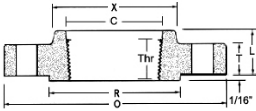
Threaded forged flange
