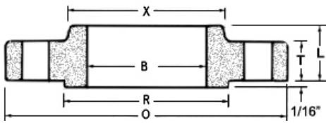
Slip on forged flange
