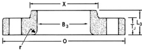
Lap Joint Weldneck forged flange
