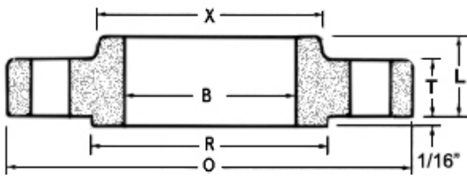
Slip on forged flange
